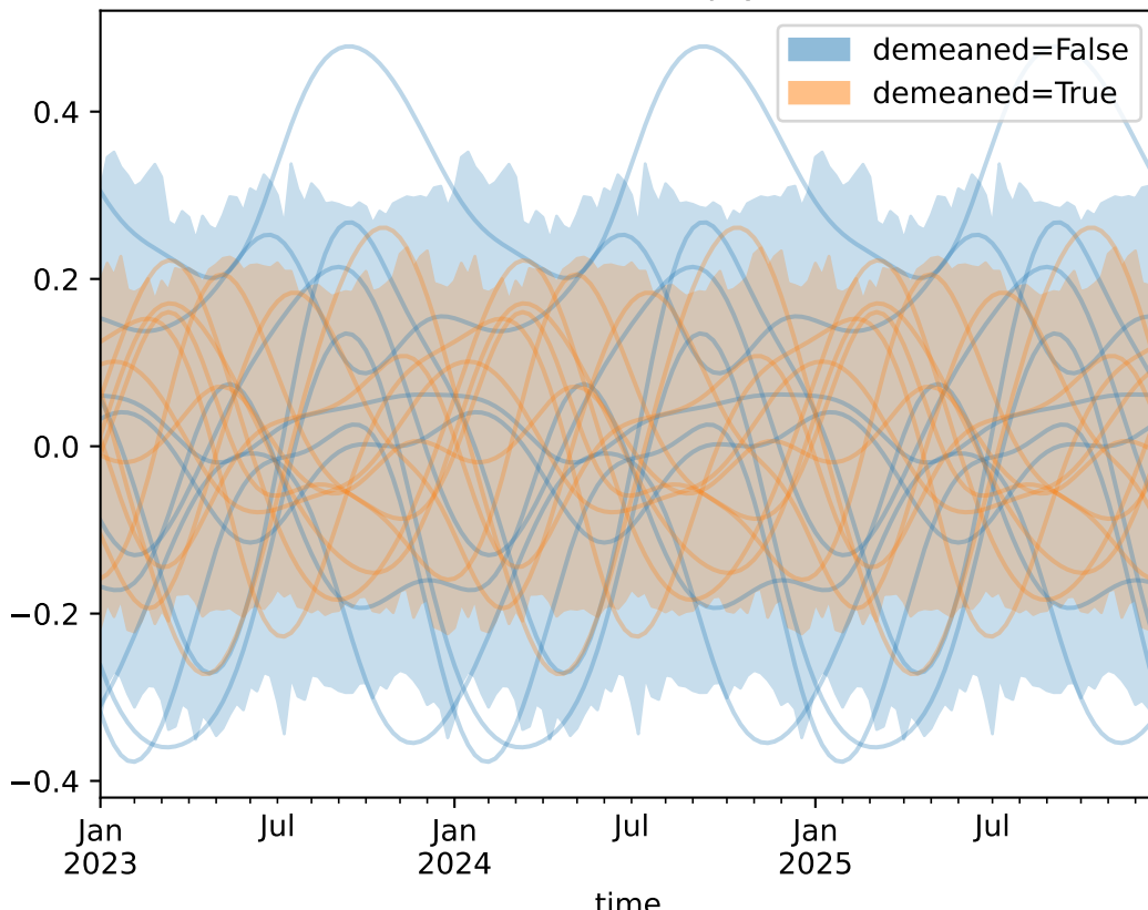
Demeaned the intercepty first basis
