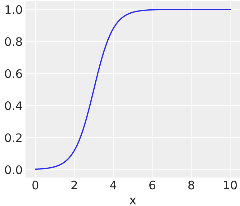
Lambda = 3
