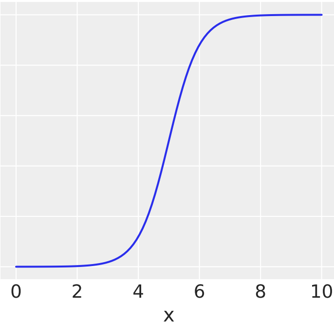
Lambda = 5
