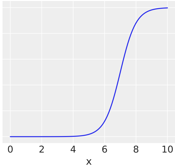
Lambda = 7
