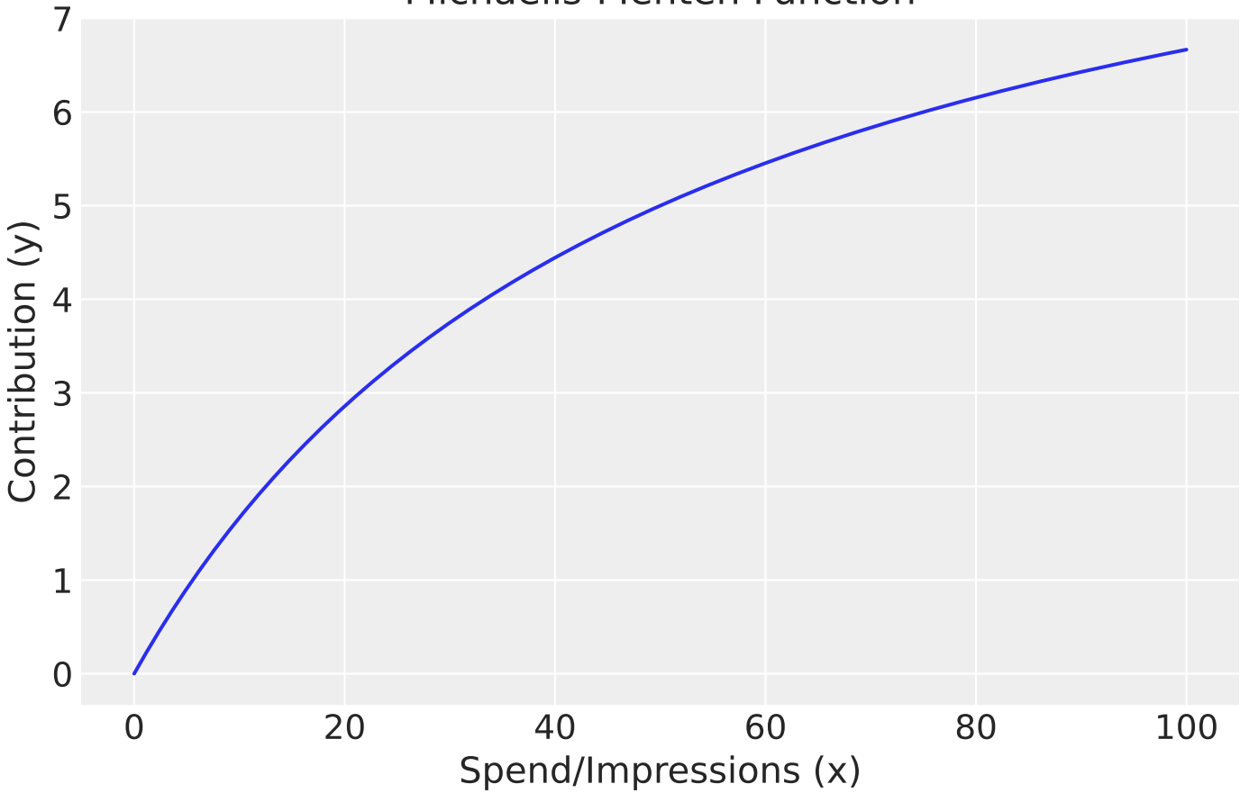
Michaelis-Menten Function
